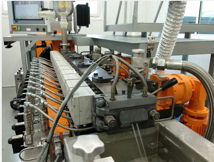
The extruder of Pilot Line 11
