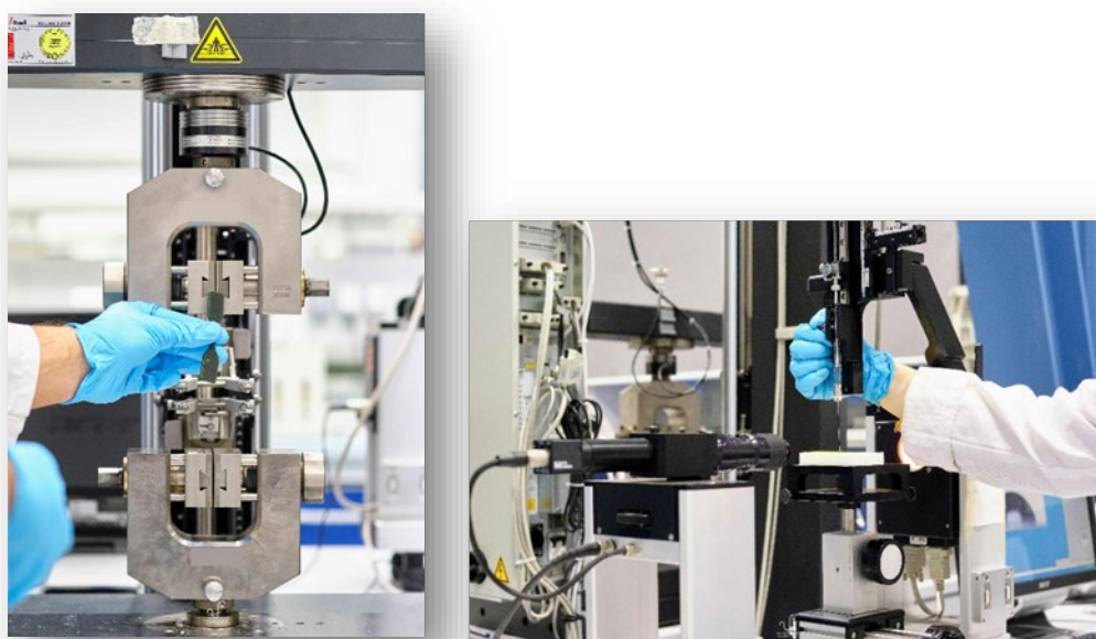
Facilities for mechanical testing of materials
