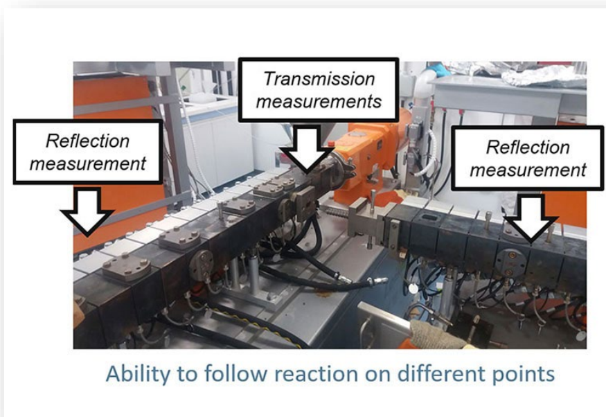
The extruder of Pilot Line 9
