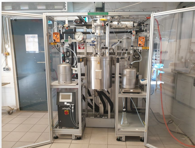
The reactor of Pilot Line 12
