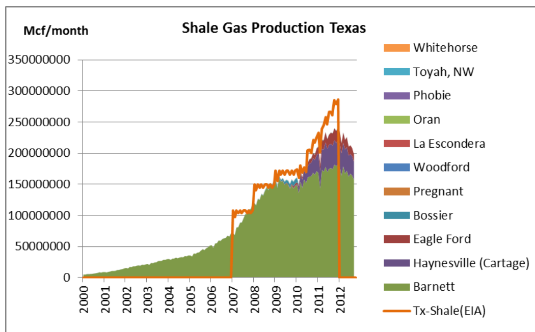
Figure 145: Shale gas production in Texas according to TRRC statistics (areas) and compared with US-EIA statistics (orange line)
