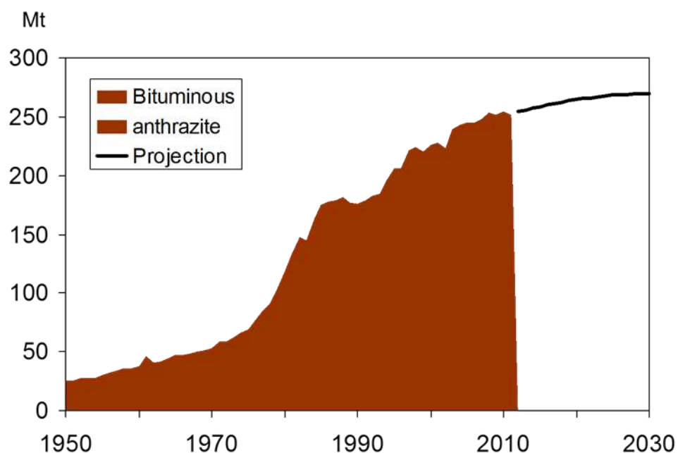
Figure 96: Coal production in South Africa
