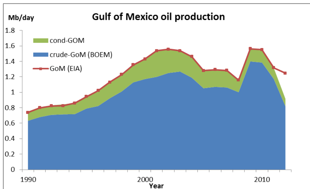
Figure 128: Oil production in the Gulf of Mexico; The US-EIA data are averages for January to October, published on 28th December 2012; the Bureau of Ocean Energy Management (BOEM) data are full year data published on 27 December 2012.
