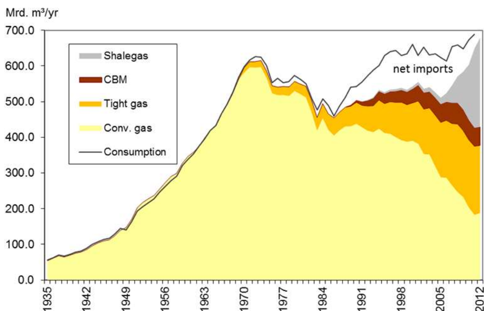
Figure 46: Gas production in USA and net imports
