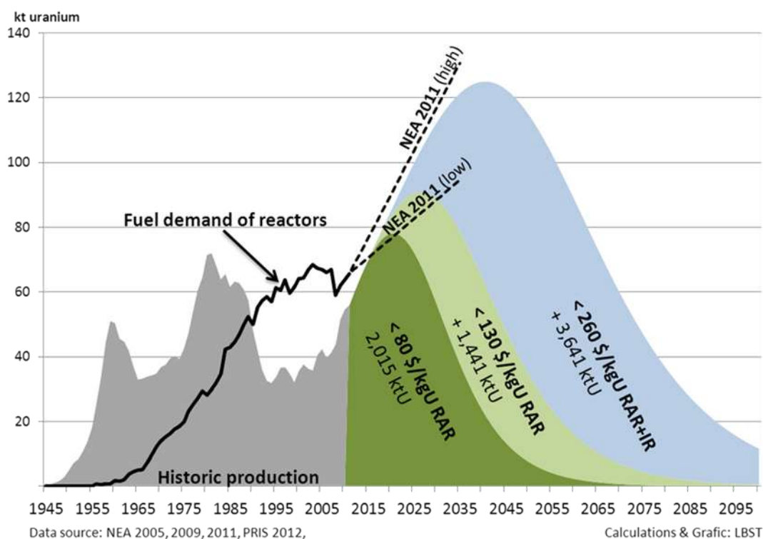
Figure 113: Historic and possible future development of uranium production and demand
