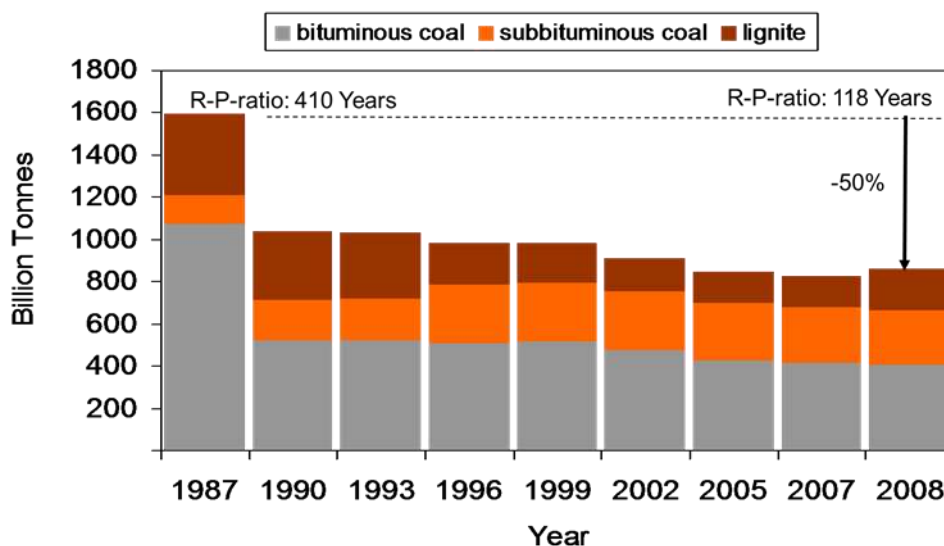
Figure 81: Historical reporting of world coal reserves (WEC 2010)
