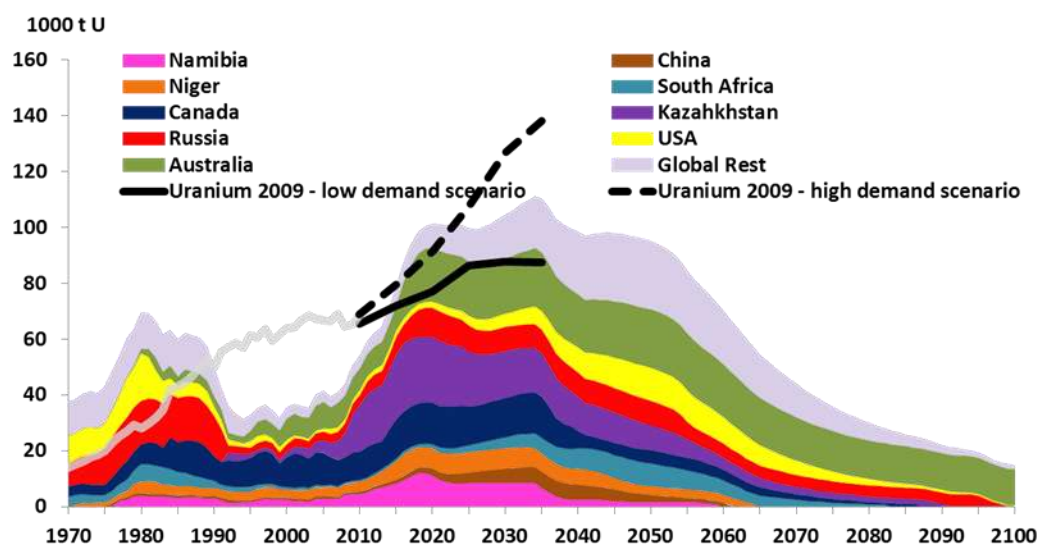
Figure 115: Historical uranium production and projection until 2100 with mine-by-mine production profiles based on Reasonably Assured Resources < 260 USD/kg and Inferred Resources < 260 USD/kg
