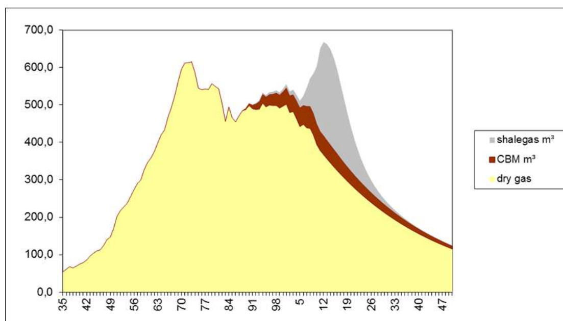
Figure 158: US Gas production and scenario based on shale gas data by Texas RRC; Other data from US-EIA
