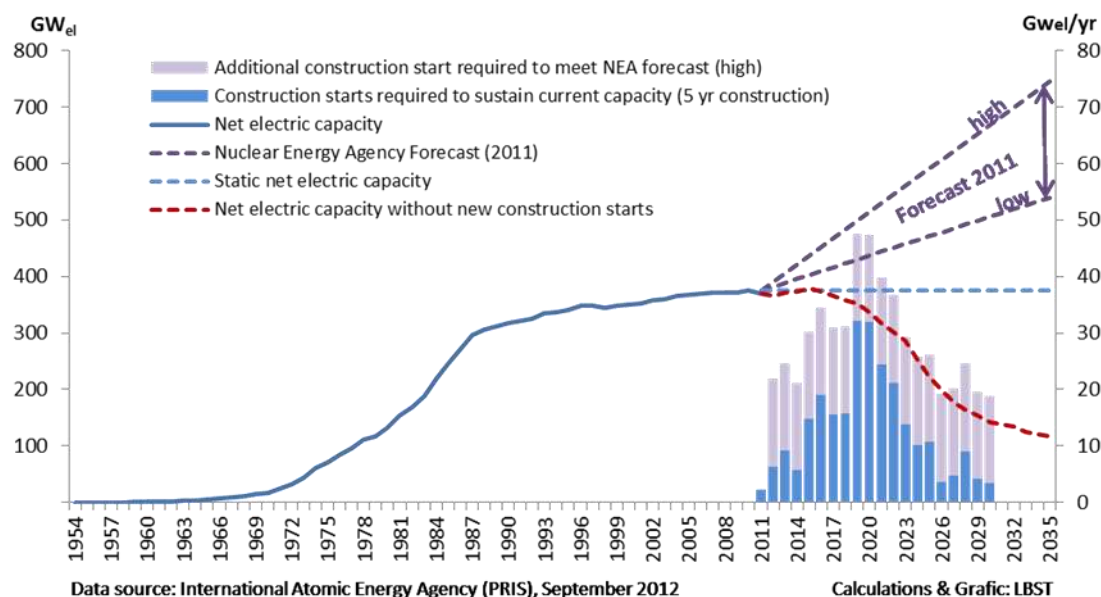
Figure 108: Required construction starts of new power plants to meet NEA forecast of nuclear capacity and to sustain current level
