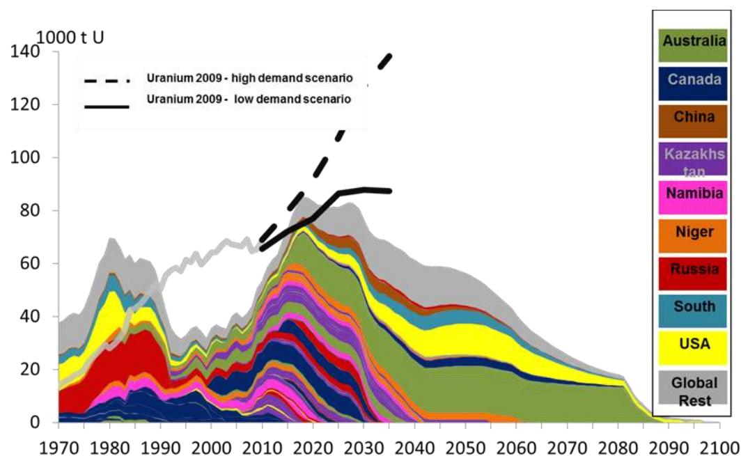
Figure 114: Historical uranium production and projection until 2100 with mine-by-mine production profiles based on Reasonably Assured Resources < 130 USD/kg
