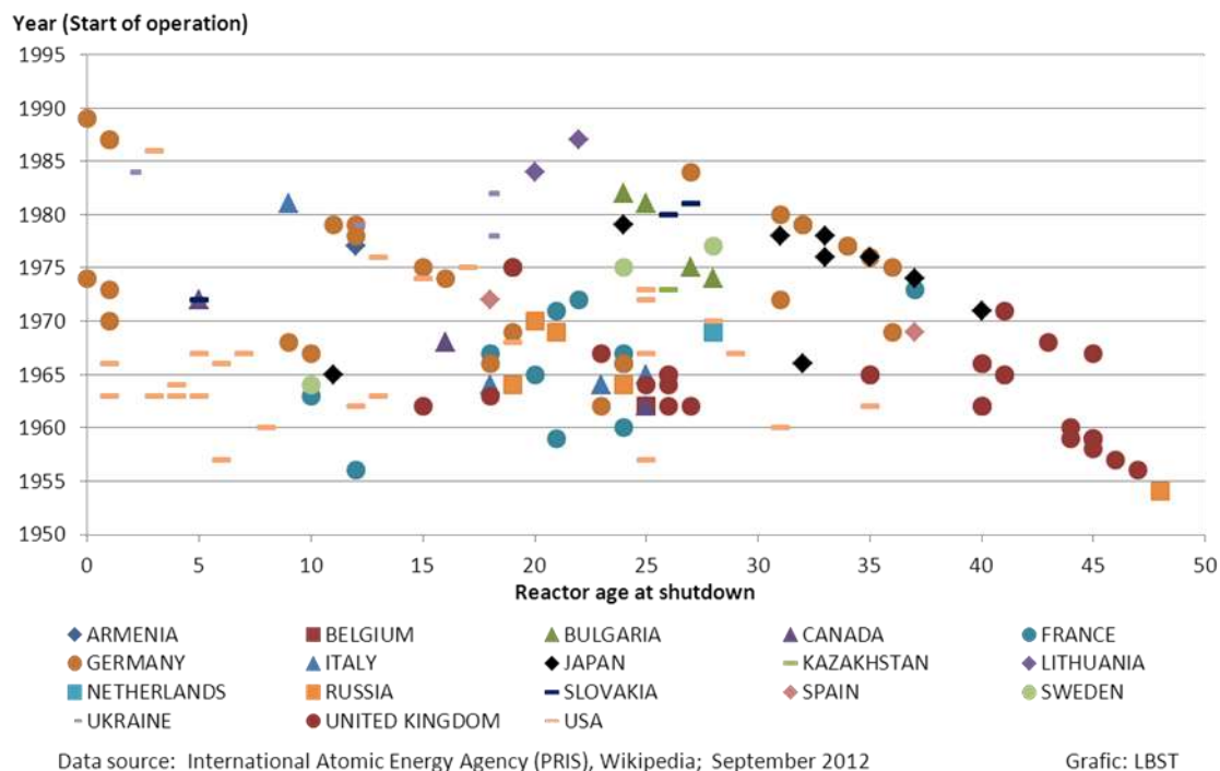
Figure 104: Age of permanent shutdown nuclear reactors at shutdown (horizontal-axis) sorted by the year operation started (vertical-axis)
