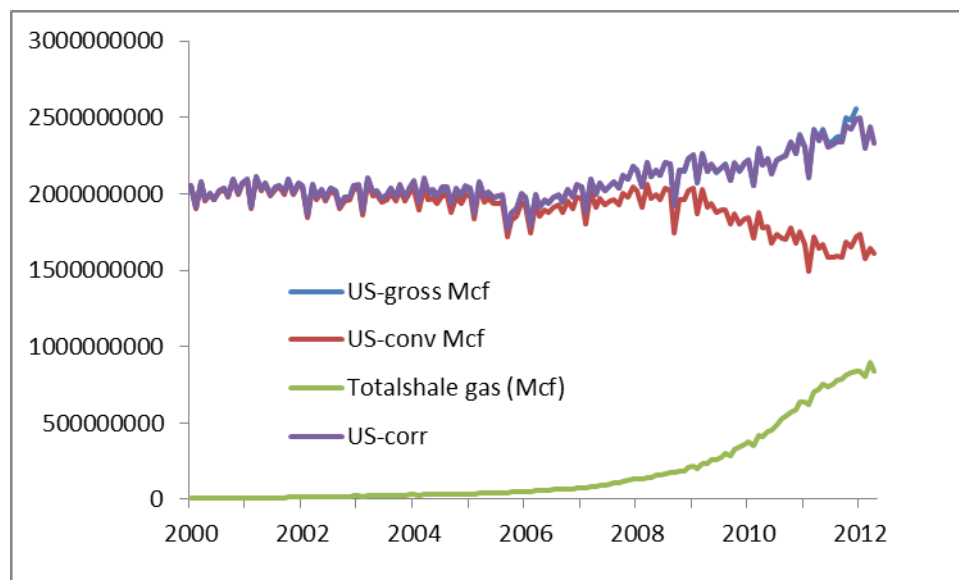
Figure 152: Domestic US gas production distinguishing conventional (including CBM and tight gas) and shale gas production.
