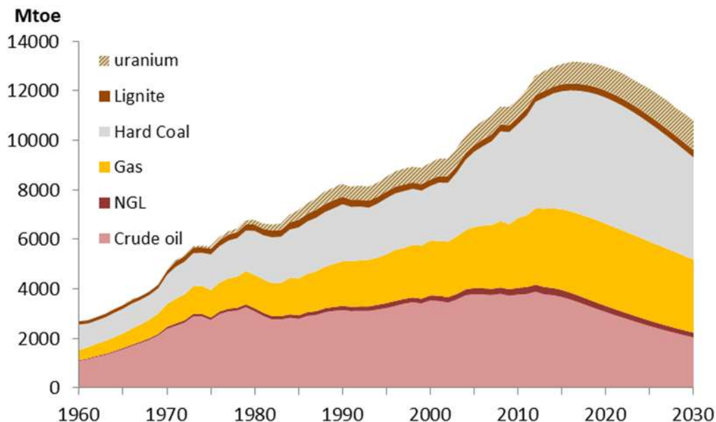
Figure 116: Fossil and nuclear energy supply from oil, NGLs, natural gas, hard coal, lignite and uranium
