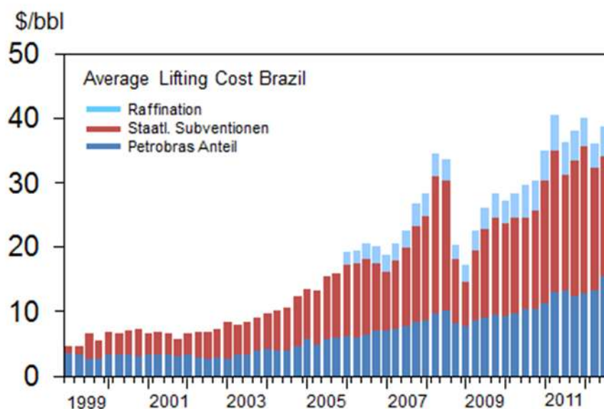
Figure 23: Quarterly average lifting cost of Petrobras (data source: Petrobras 2013)
