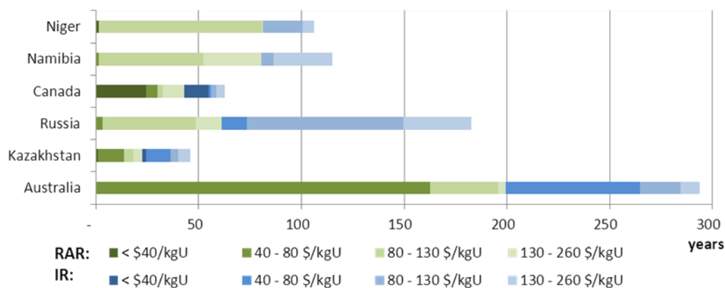
Figure 111: Resource to production ratio for the 6 biggest uranium producers at 2010s production volume
