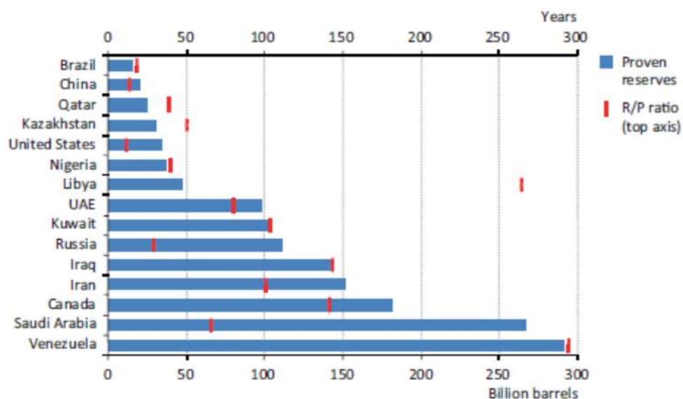
Figure 45: Reserves and Resources according to WEO 2012 (WEO 2012)
