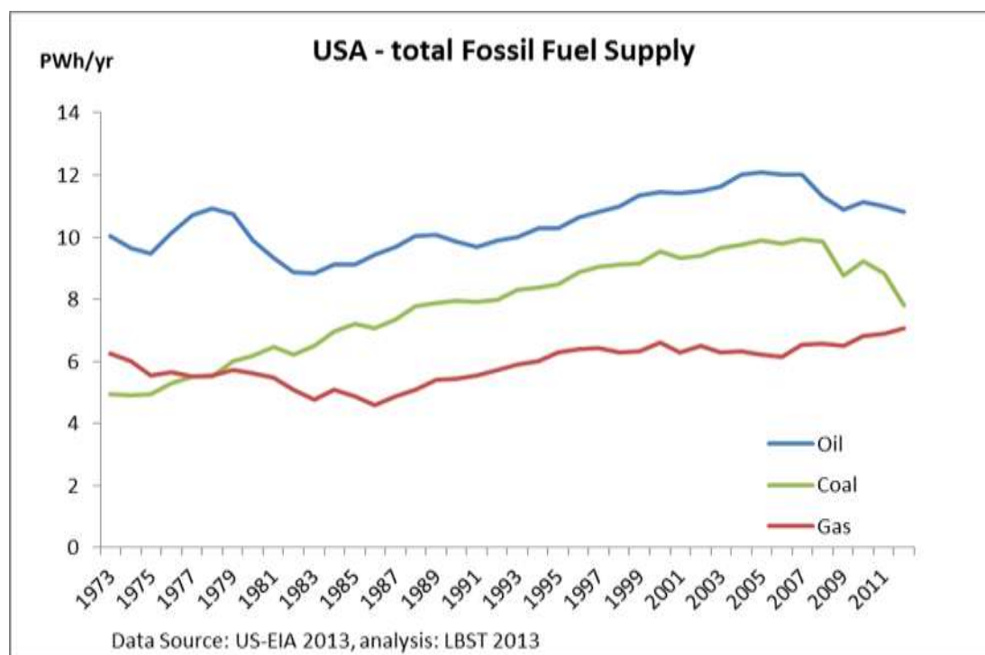
Figure 117: Fossil fuel consumption in the USA between 1973 and 2012; data for 2012 are extrapolated from monthly data until Sep (coal), Oct (gas) and Nov (oil) (Data source US-EIA 2013)
