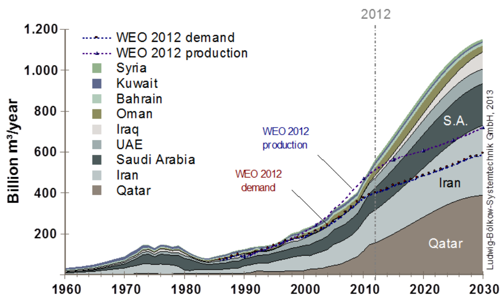
Figure 75: Natural gas production in Middle East
