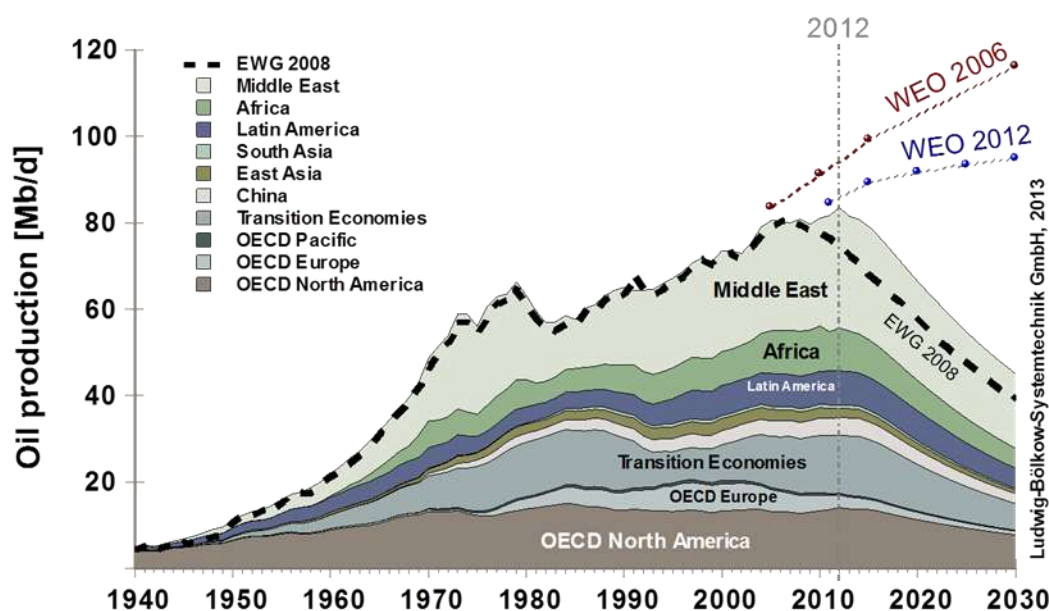
Figure 24: World oil supply according to EWG scenario 2013
