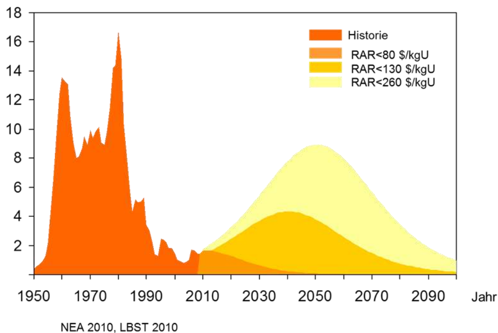
Figure 167: Various production scenarios of uranium in the USA based on different classes of resources
