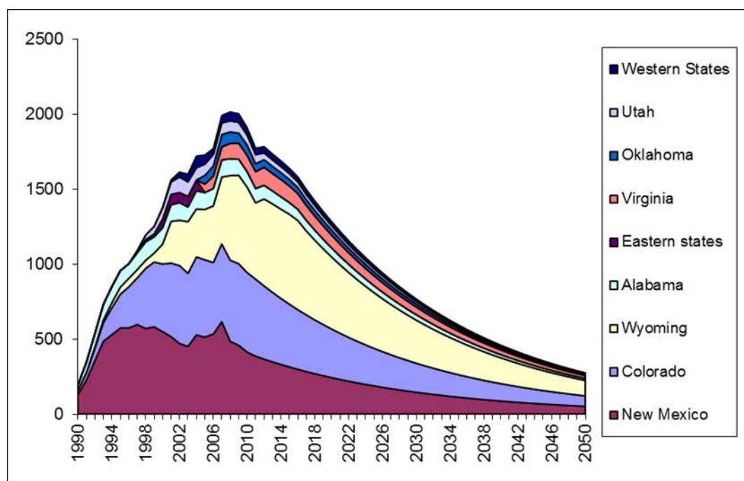
Figure 50: Historical production of coal bed methane and scenario calculation until 2050
