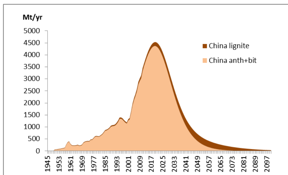
Figure 93: Coal production in China
