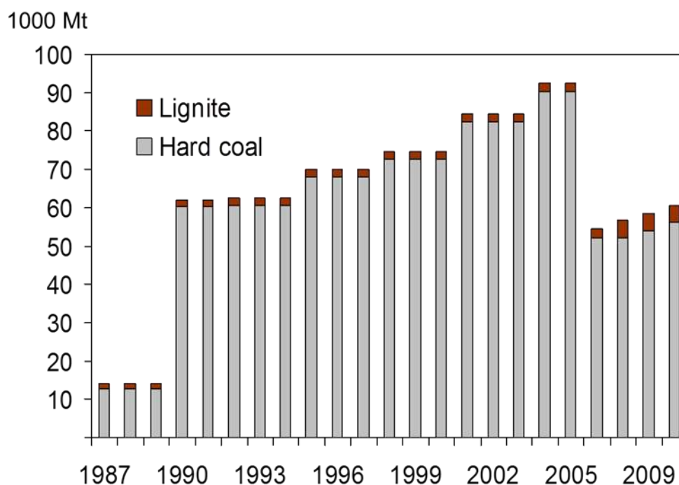
Figure 87: reported coal reserves of India (WEC 2010, BP 2012)
