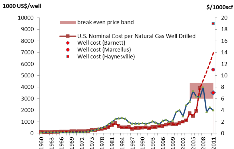
Figure 48: Cost of natural gas wells drilled and natural gas well head price (Source: US-EIA 2012, Berman 2012, Baihly 2011)
