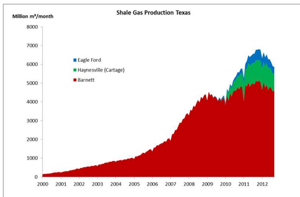
Figure 53: Shale gas production in Texas until Nov 2012 (RRC)
