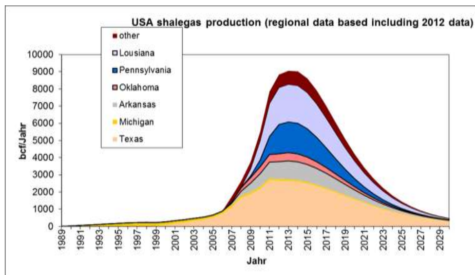
Figure 56: Scenario calculation for shale gas development in USA until 2030.
