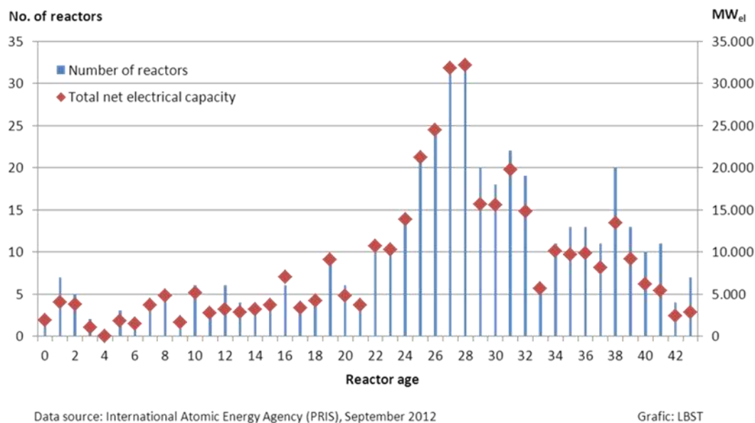
Figure 105: Age of the operational nuclear power plant fleet (Status 2012)
