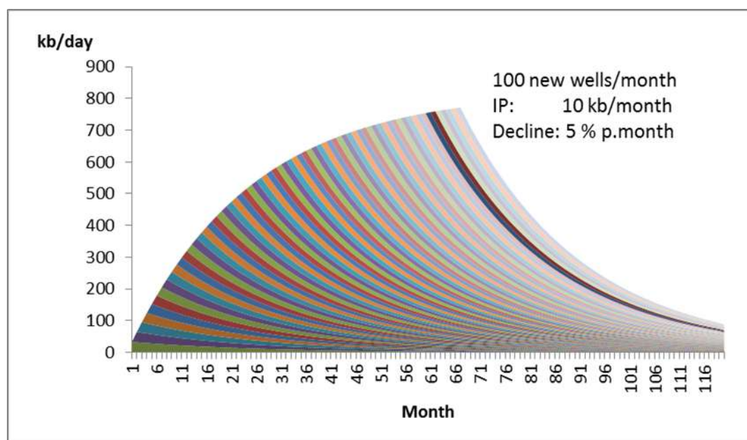
Figure 125: Theoretical model calculation of tight oil well developments
