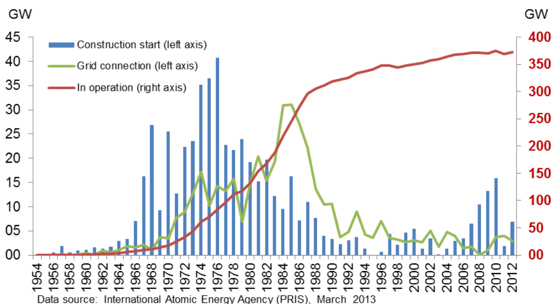
Figure 103: Construction start, grid connection and accumulated net electric capacity of nuclear power plants at world level
