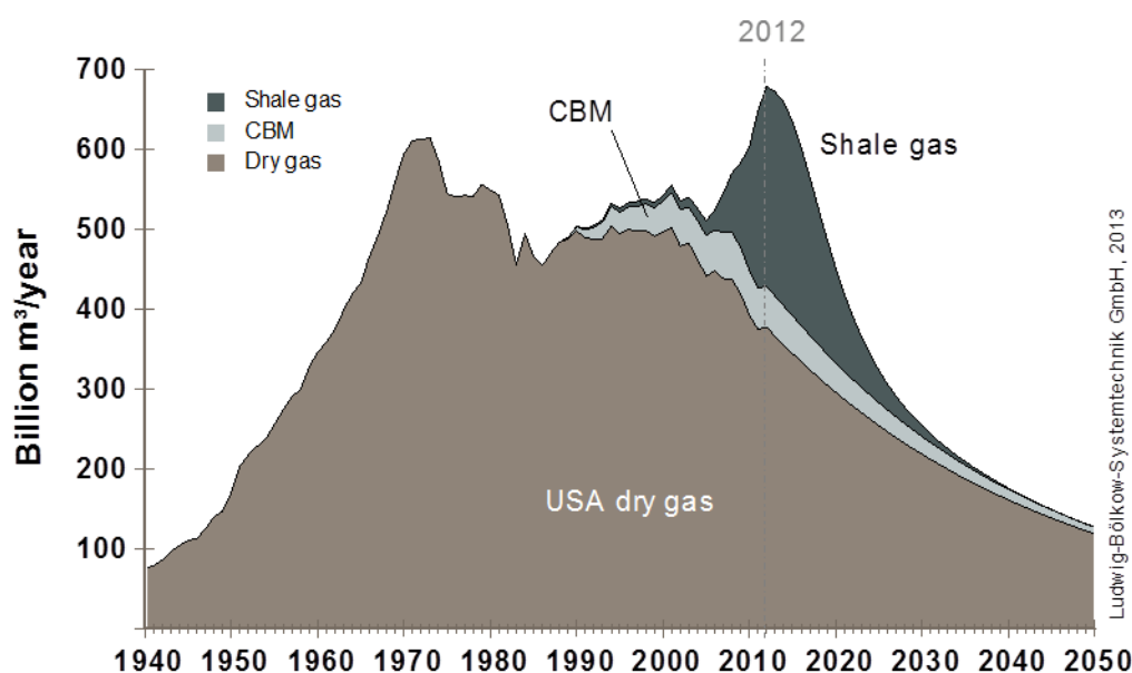
Figure 57: US gas production scenario until 2050
