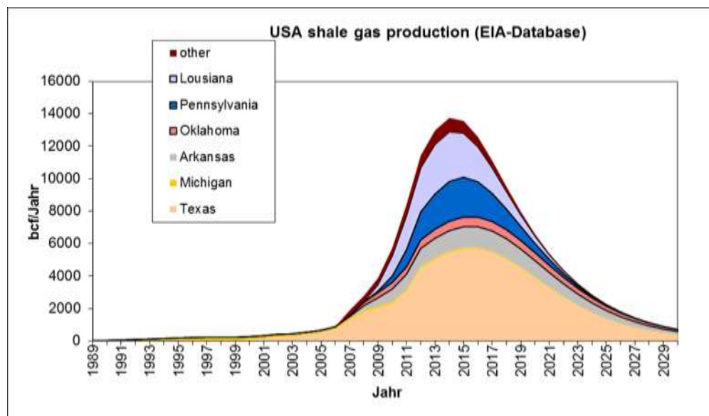
Figure 155: Development of natural gas production from shale gas deposits in the USA (high case)
