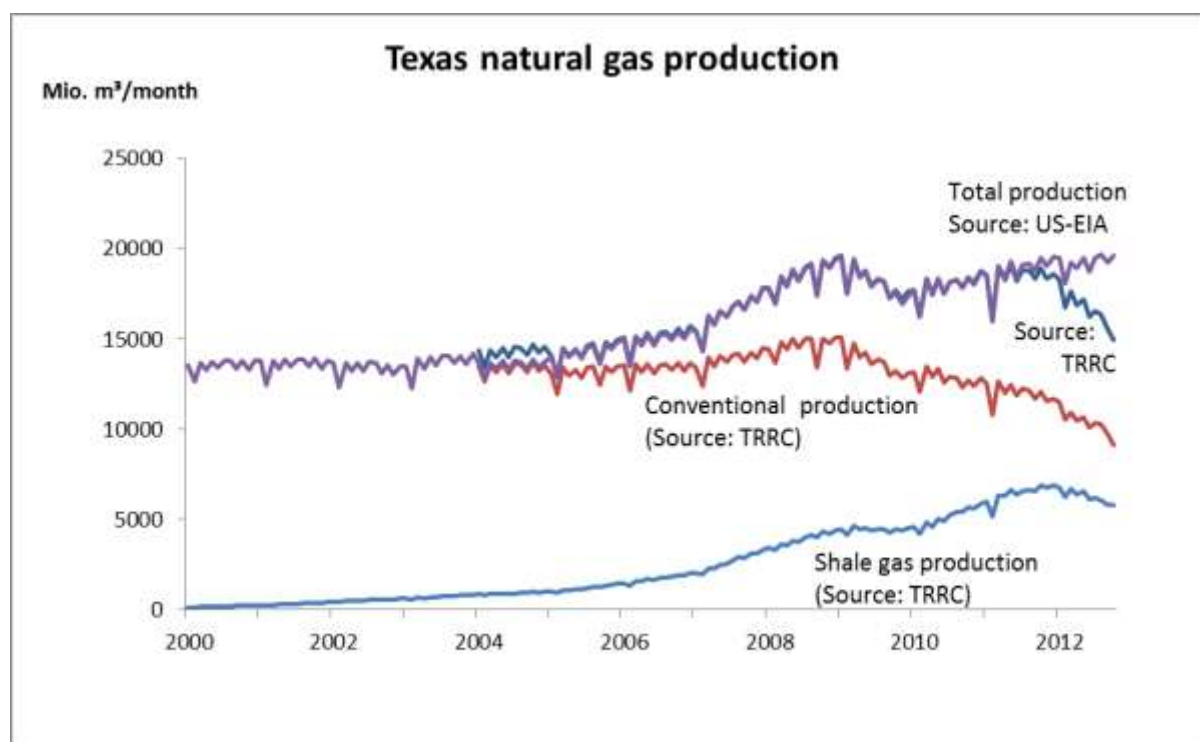
Figure 144: Natural gas production in Texas according US-EIA and compared with detailed statistics by Texas Railroad Commission statistics
