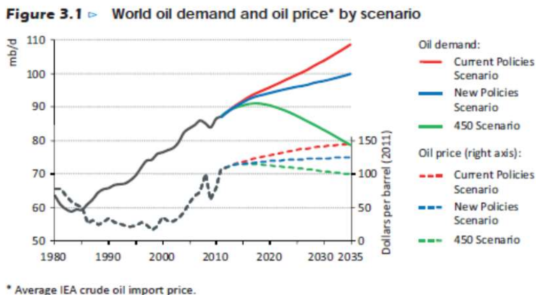
Figure 39: World oil demand according to WEO 2012. (WEO 2012)
