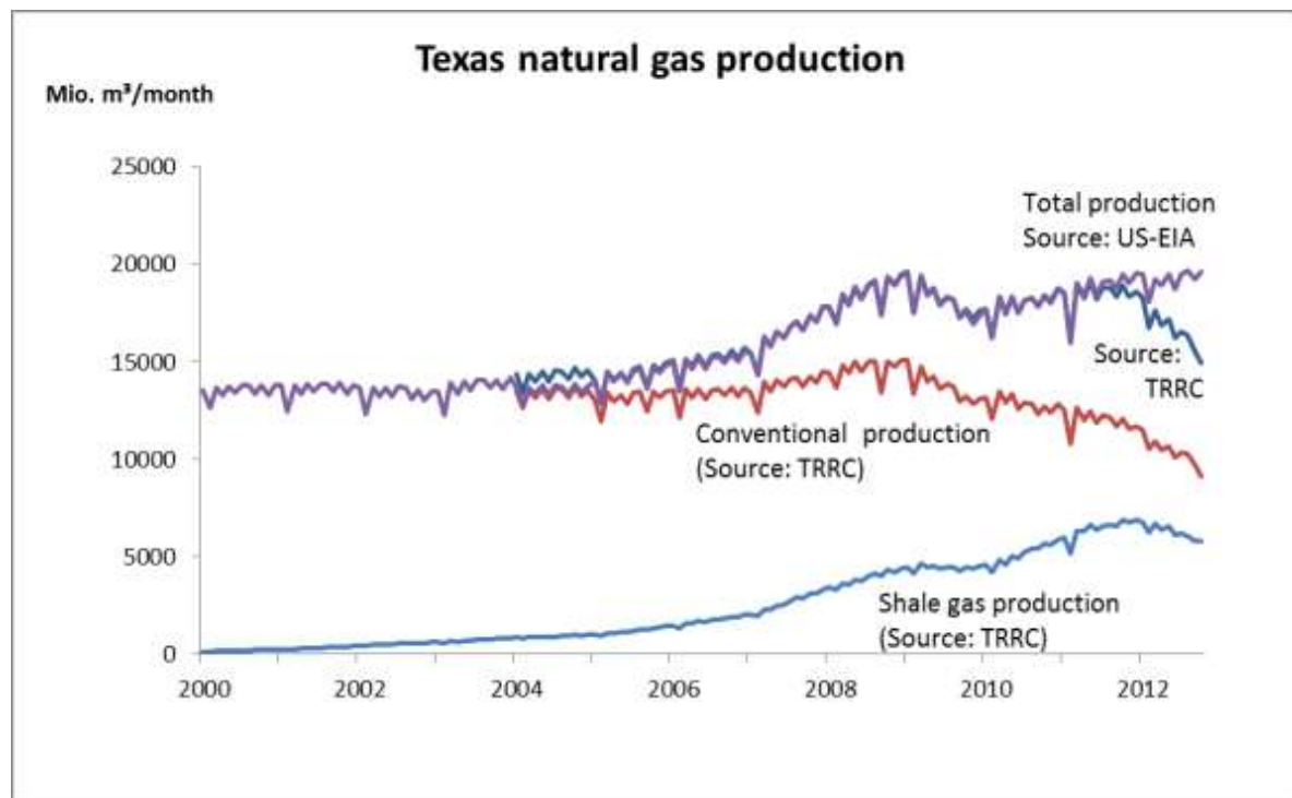
Figure 54: Total gas production in Texas; Reporting discrepancies between Texas Railroad Commission and US-Energy Information Administration
