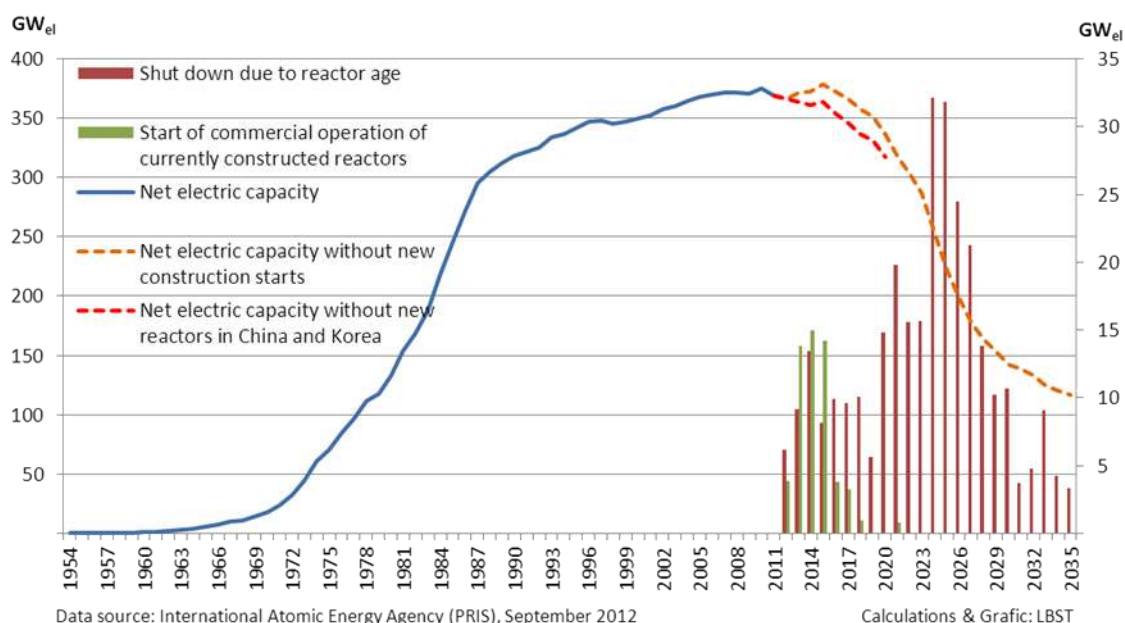
Figure 107: Development of the installed net electrical capacity if no new NPP constructions start.
