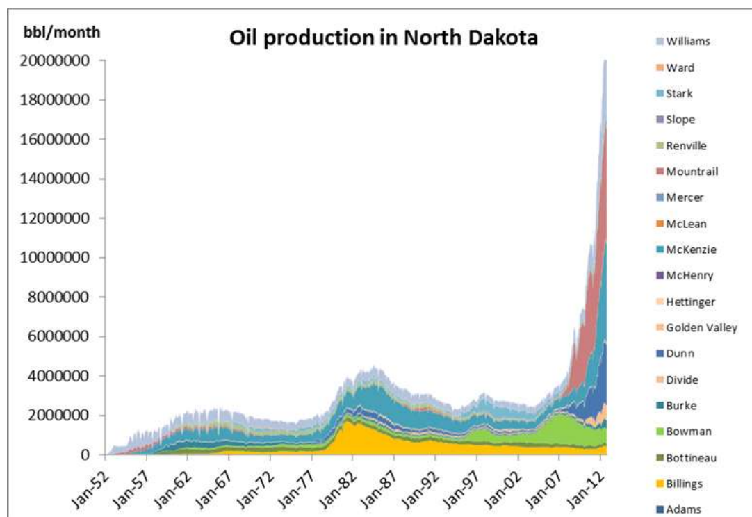
Figure 123: Crude oil production in individual counties in North Dakota. Most counties are already showing a decline. The huge production increase only takes place in four counties.(Source: NDG 2013)
