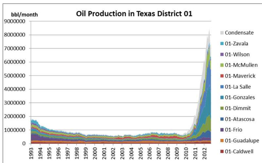
Figure 121: Oil production of individual counties inside Texas District 01 (Source: TRRC Query 2013)
