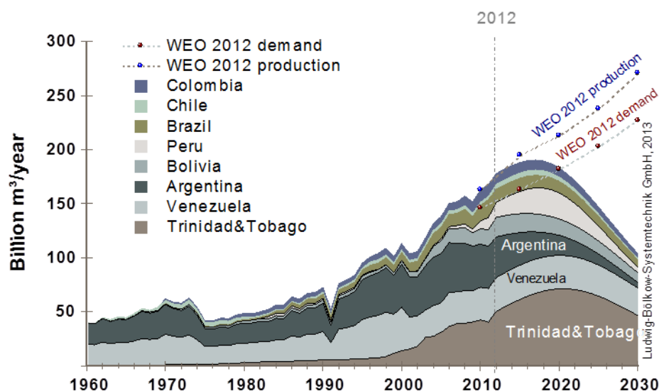
Figure 79: Natural gas production in Latin America
