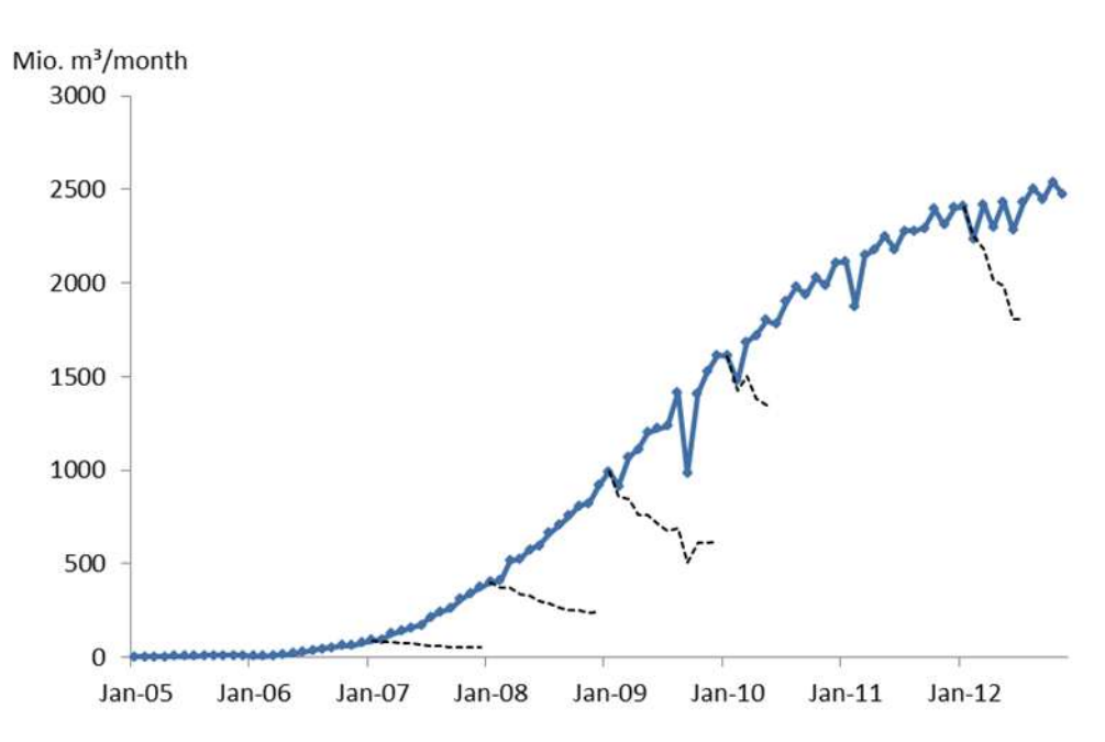
Figure 52: Gas production from the Fayetteville Shale in Arkansas
