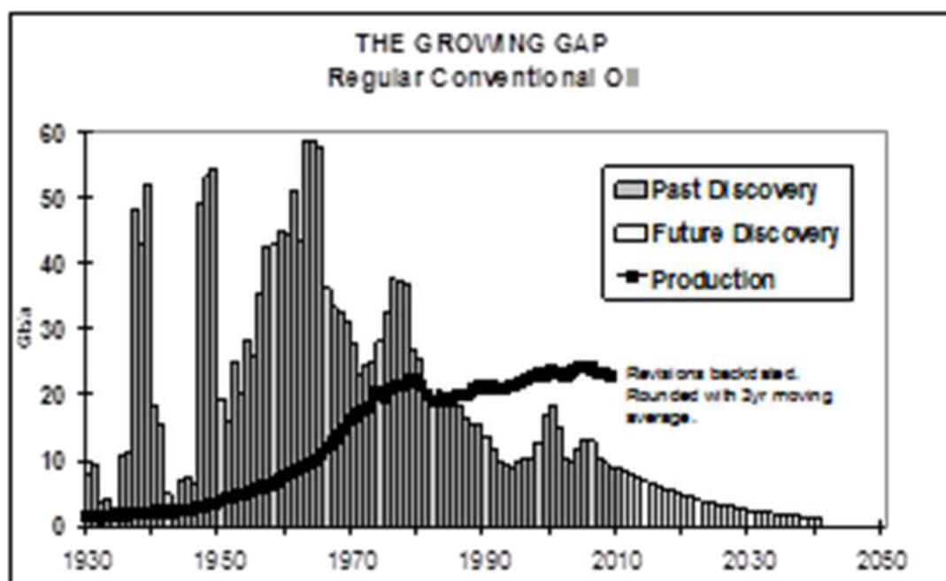
Figure 2: Historical discovery pattern of conventional oil fields and projection until 2040. (Campbell 2012)
